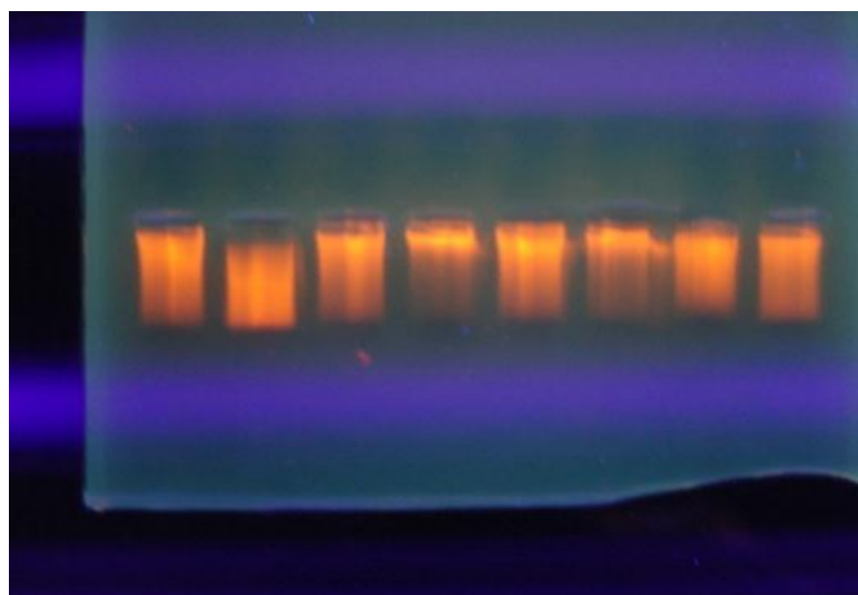
Figures (1, 2) show DNA extraction and amplification of T. vaginalis after Electrophoresis in 0.2 % of agarose gel, the sample 1, 3, 4 show positive results, 2 show negative results, M is DNA Ladder to compare results
